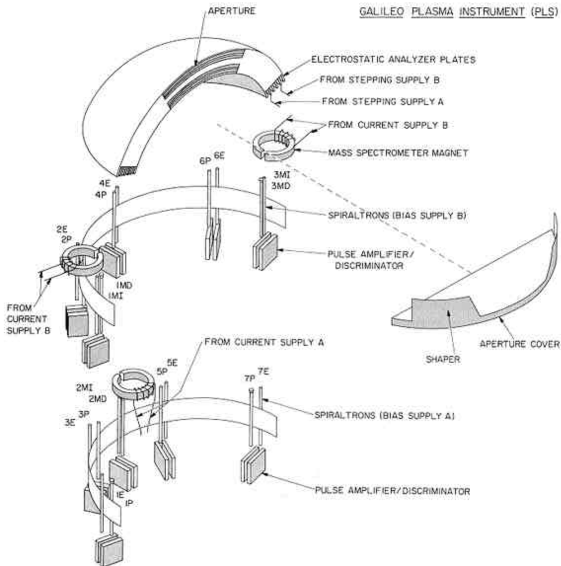
Fig. 1. An exploded view of the electrostatic analyzers, miniature mass spectrometers, and sensors of the plasma instrumentation (PLS) for the Galileo Mission.
