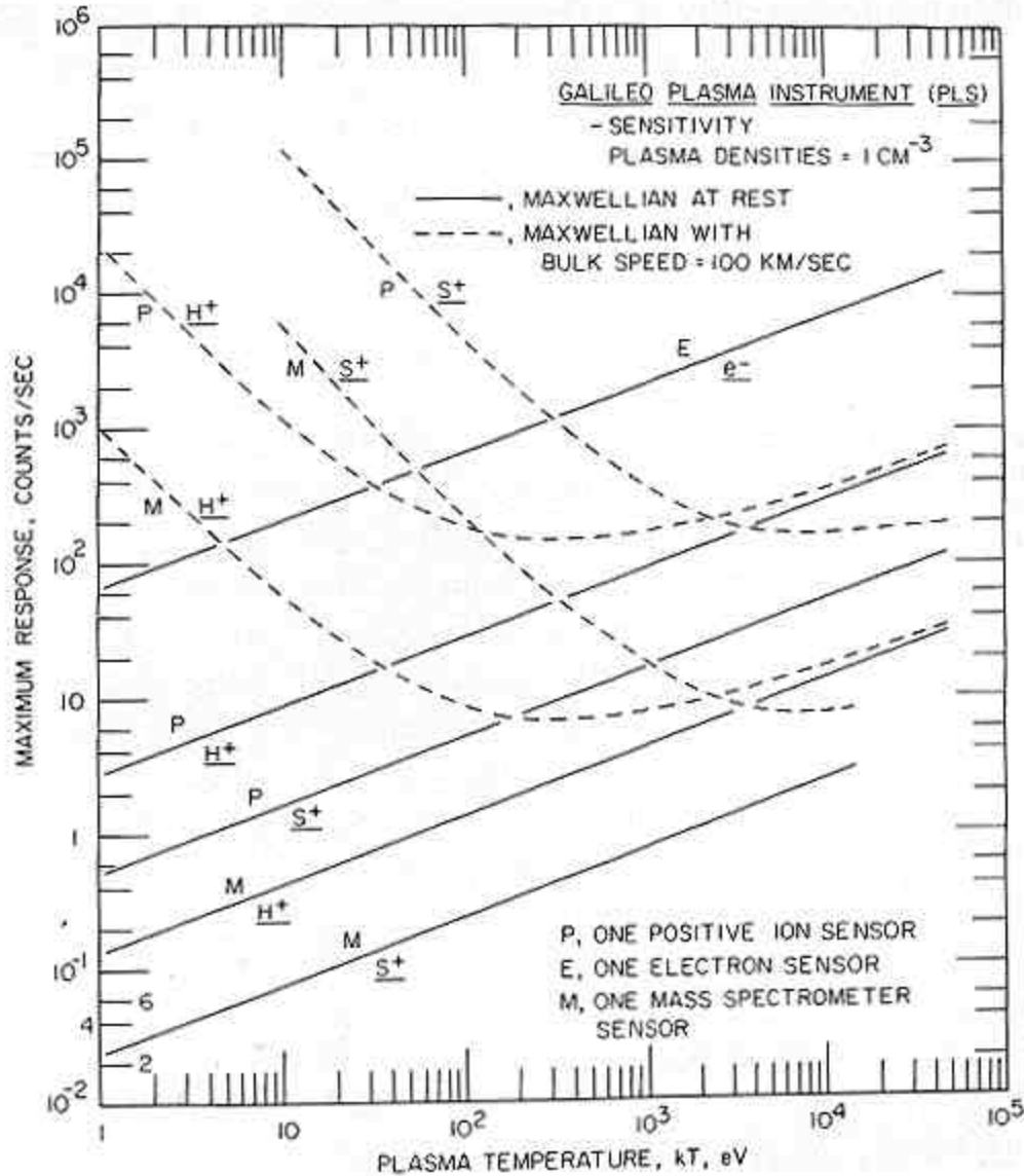
Fig. 8. Maximum responses of several individual sensors to a Maxwellian plasma distribution as a function of plasma temperature. Responses to \text{H}^+ and \text{S}^+ plasmas at rest and with bulk flow speed 100 \text{ km s}^{-1} are shown. The densities of electron and ion plasmas are each taken as 1 \text{ cm}^{-3} .
