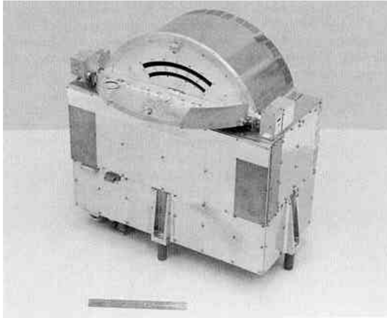
Fig. 4. Photograph of the plasma instrument. The two arc-shaped openings are the apertures for the two sets of electrostatic analyzers. A 6-inch ruler is shown for comparisons.
