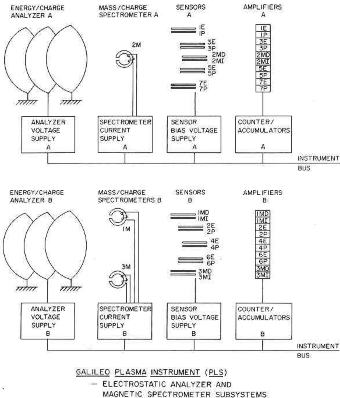
Fig. 9. Block diagram for the two analyzers, A and B, in the plasma instrument.
