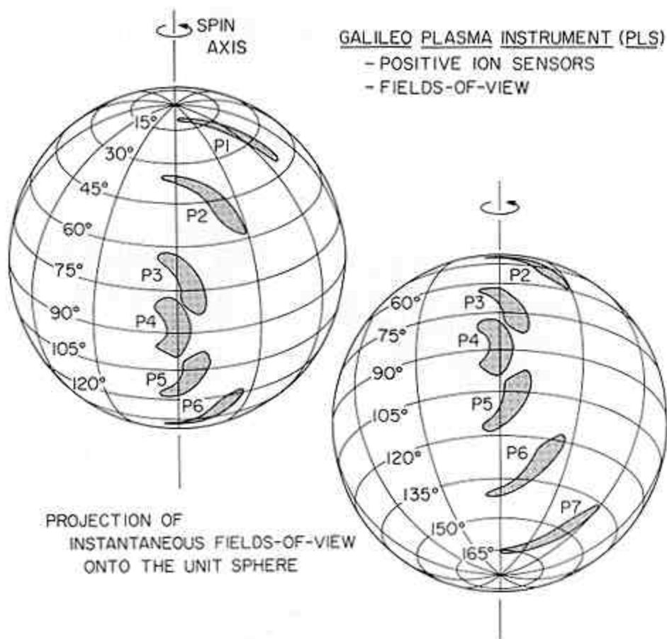
Fig. 2. The instantaneous fields-of-view for the seven positive ion sensors as projected onto the unit sphere. Rotation of the spacecraft spinning section provides coverage of 80% of the unit sphere for ion velocity vectors. The coverage of this solid angle with the seven electron sensors is similar.
