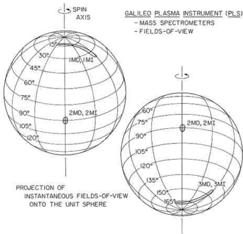
Fig. 3. The instantaneous fields-of-view for the three mass spectrometers as projected onto the unit sphere.
