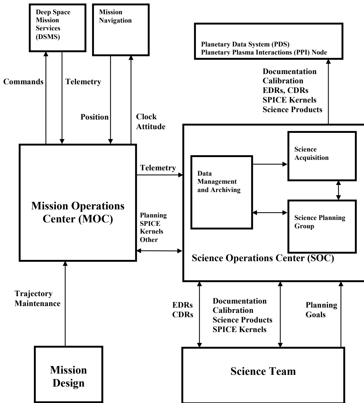
Figure 4: Data flow.
